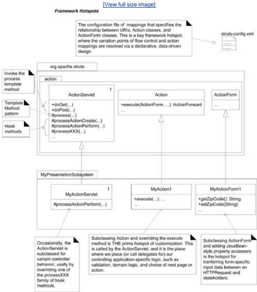
Figure 3. Struts framework hotspots.
