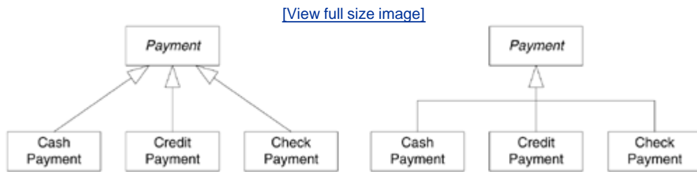
Figure 32.2. Class hierarchy with separate and shared arrow notations.
