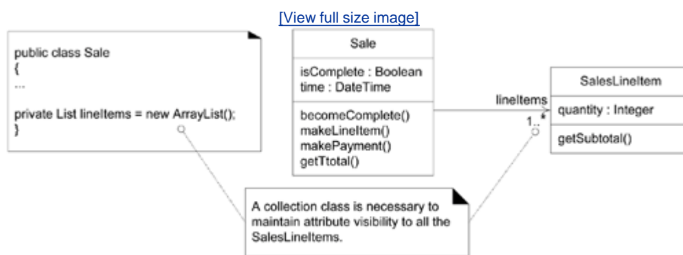
Figure 20.5. Adding a collection.
