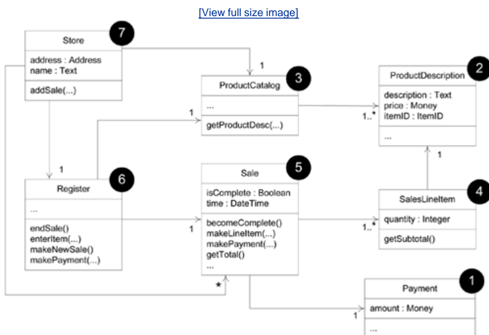
Figure 20.7. Possible order of class implementation and testing.
