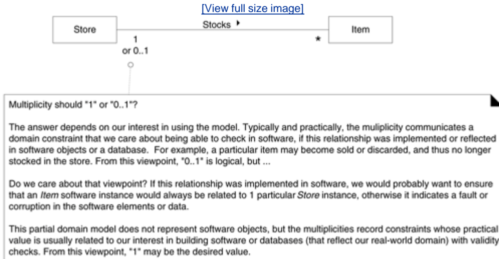
Figure 9.15. Multiplicity is context dependent.
