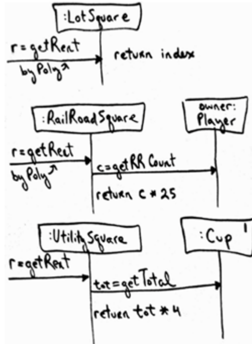
Figure 35.28. Polymorphic getRent methods.
