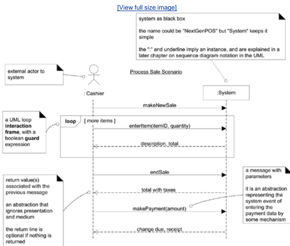
Figure 10.2. SSD for a Process Sale scenario.
