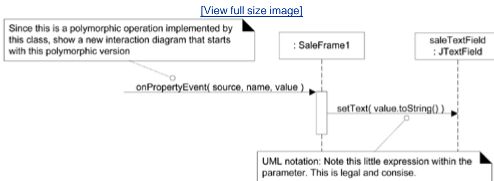
Figure 26.25. The subscriber SaleFrame1 receives notification of a published event.
