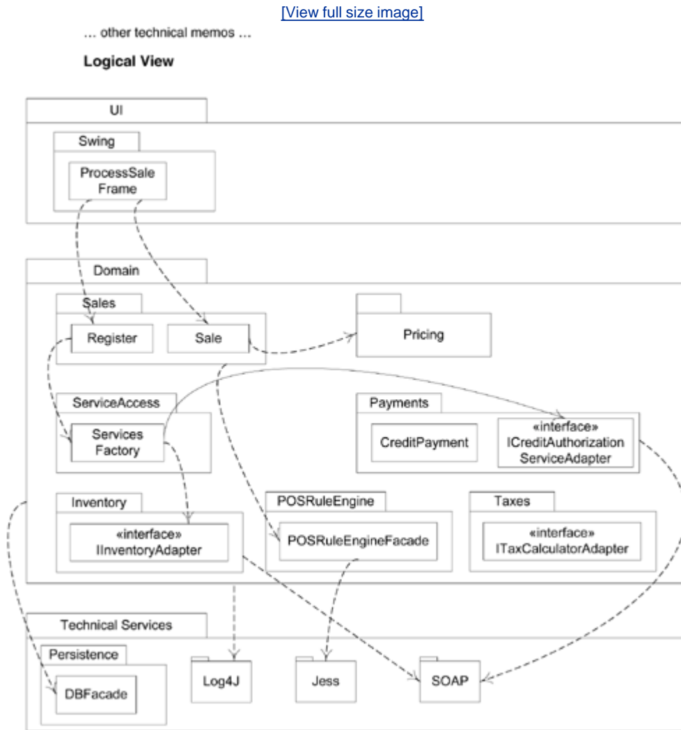
Figure 1. Package diagram of the logical view.
