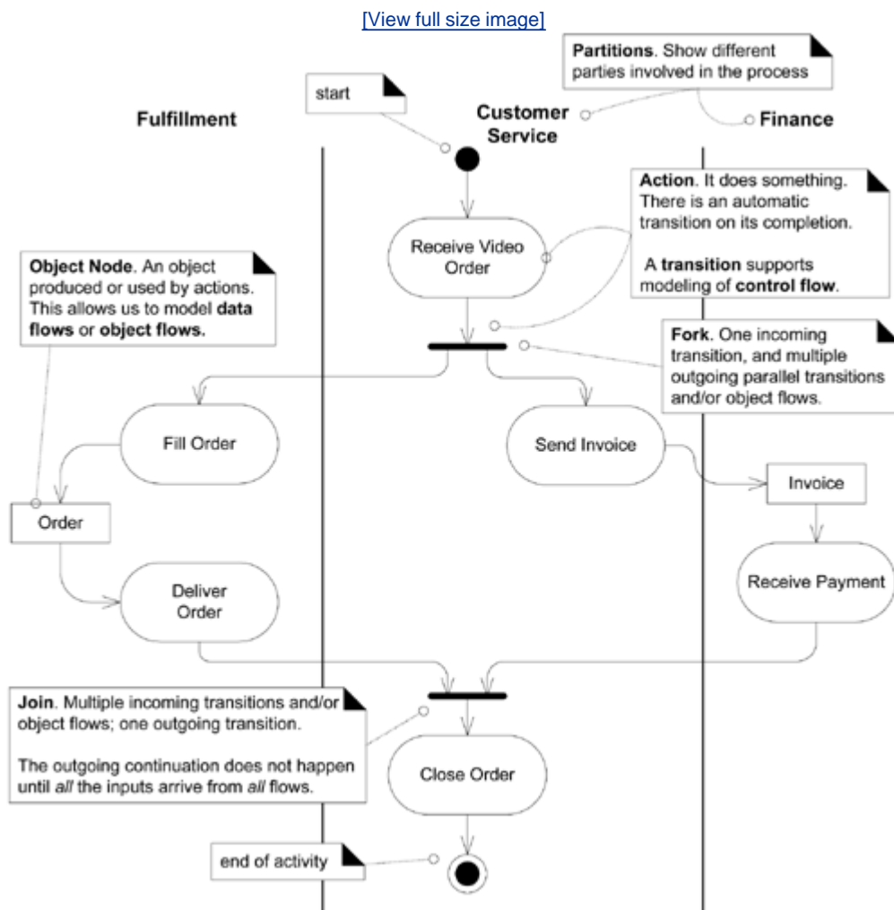
Figure 28.1. Basic UML activity diagram notation.
