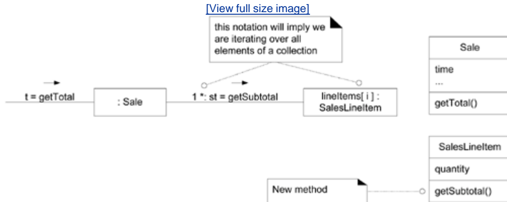
Figure 17.16. Calculating the Sale total.
