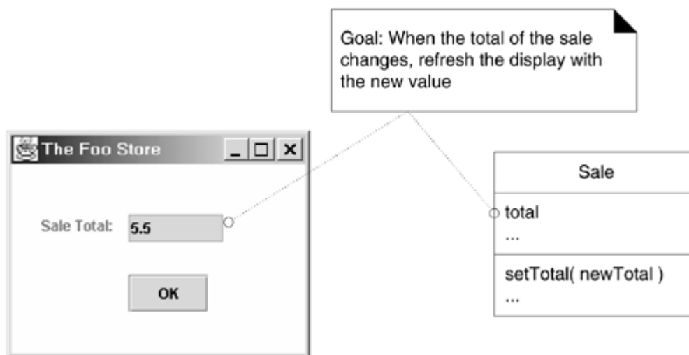
Figure 26.21. Updating the interface when the sale total changes.
