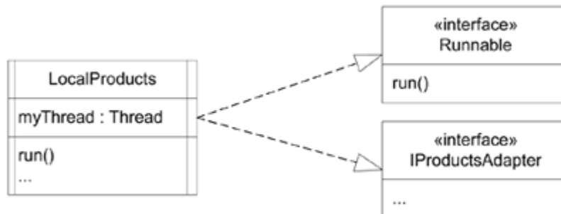
Figure 35.8. Active class notation.
