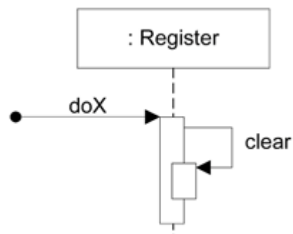
Figure 15.9. Messages to "this."
