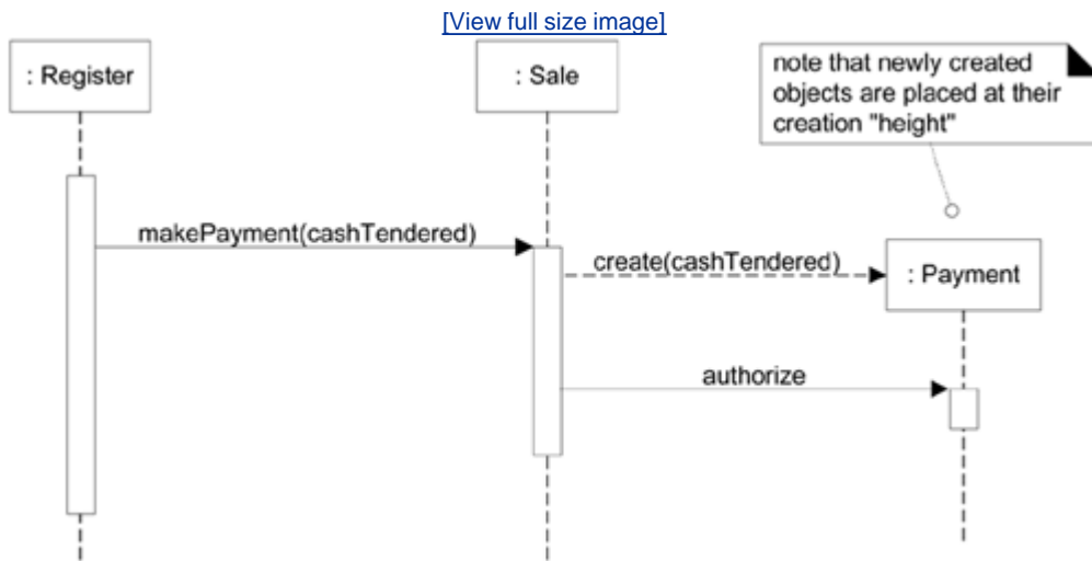
Figure 15.10. Instance creation and object lifelines.
