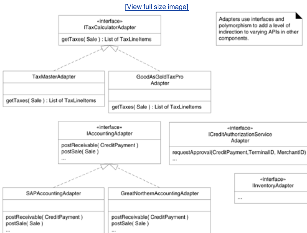
Figure 26.1. The Adapter pattern.
