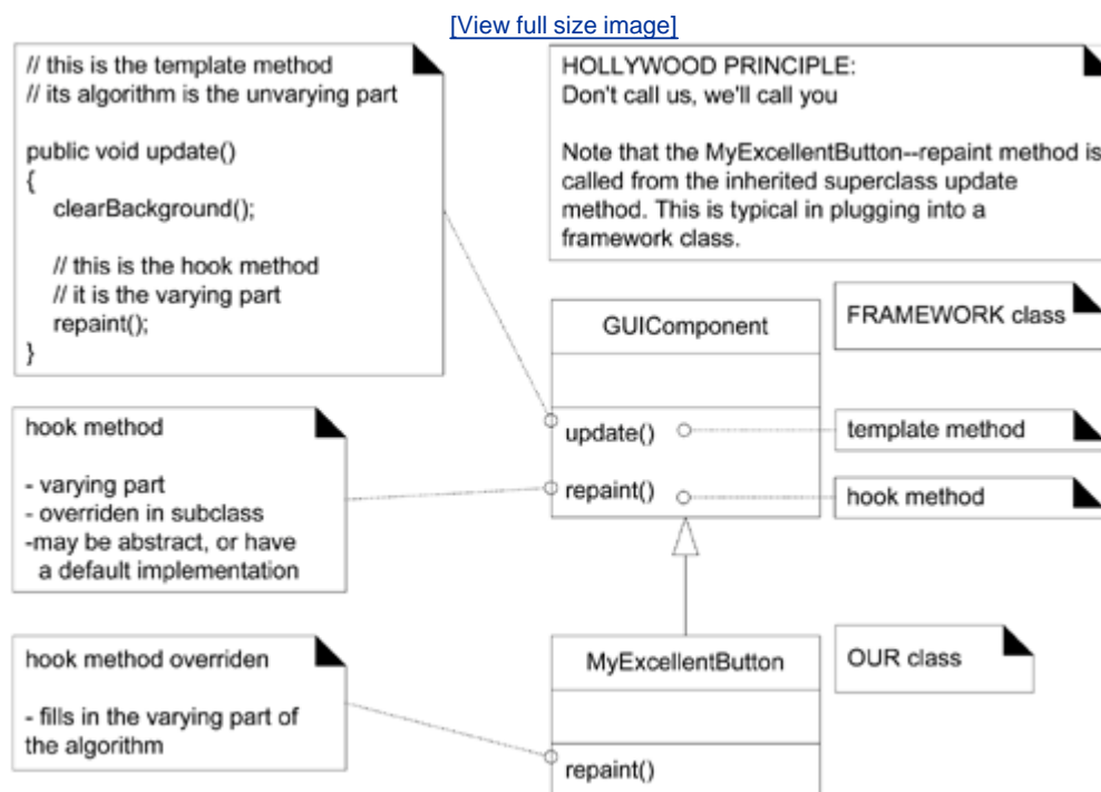
Figure 38.6. Template Method pattern in a GUI framework.
