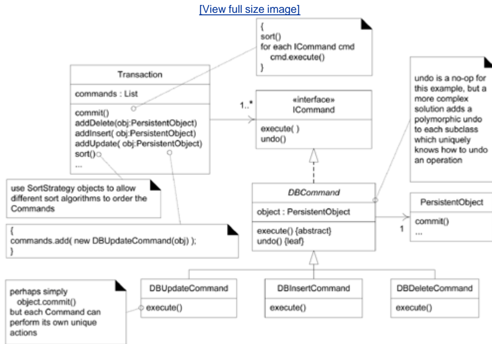
Figure 38.15. Commands for database operations.
