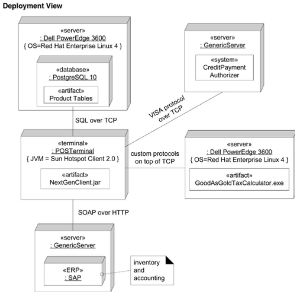
Figure 2. Deployment view.
