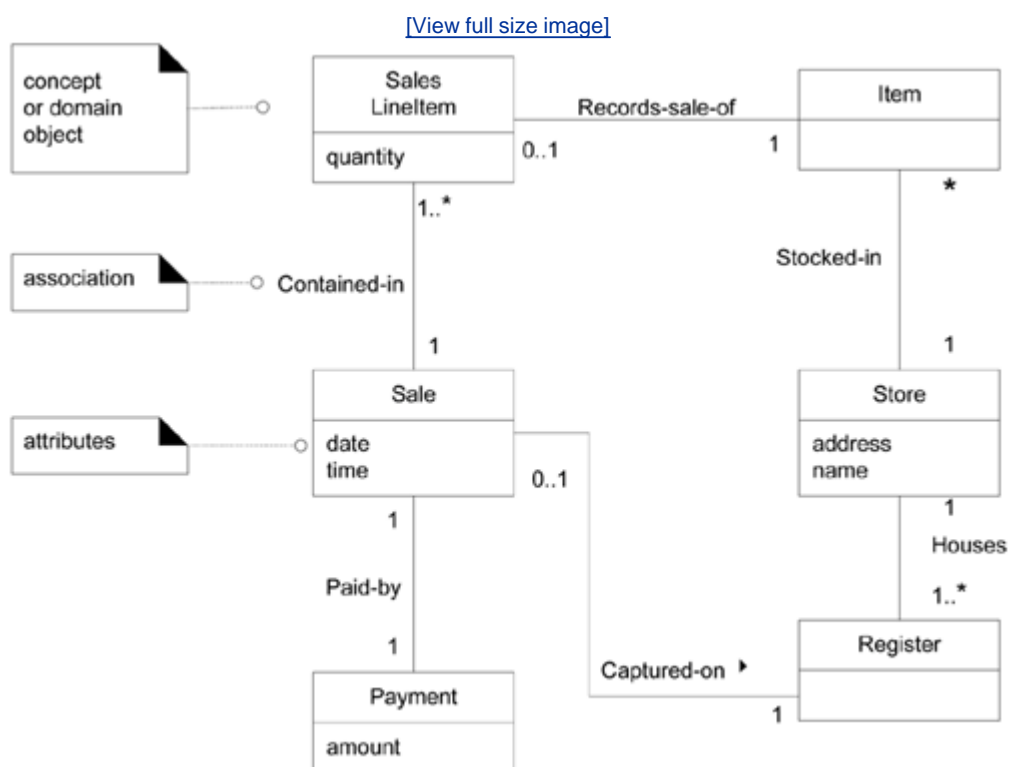
Figure 9.2. Partial domain model a visual dictionary.
