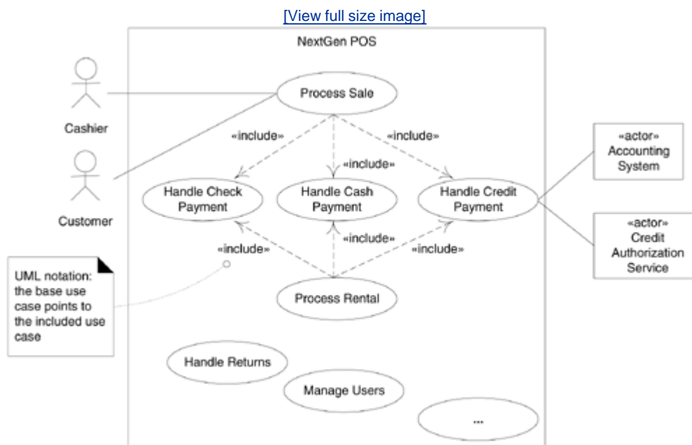
Figure 30.1. Use case include relationship in the Use-Case Model.
