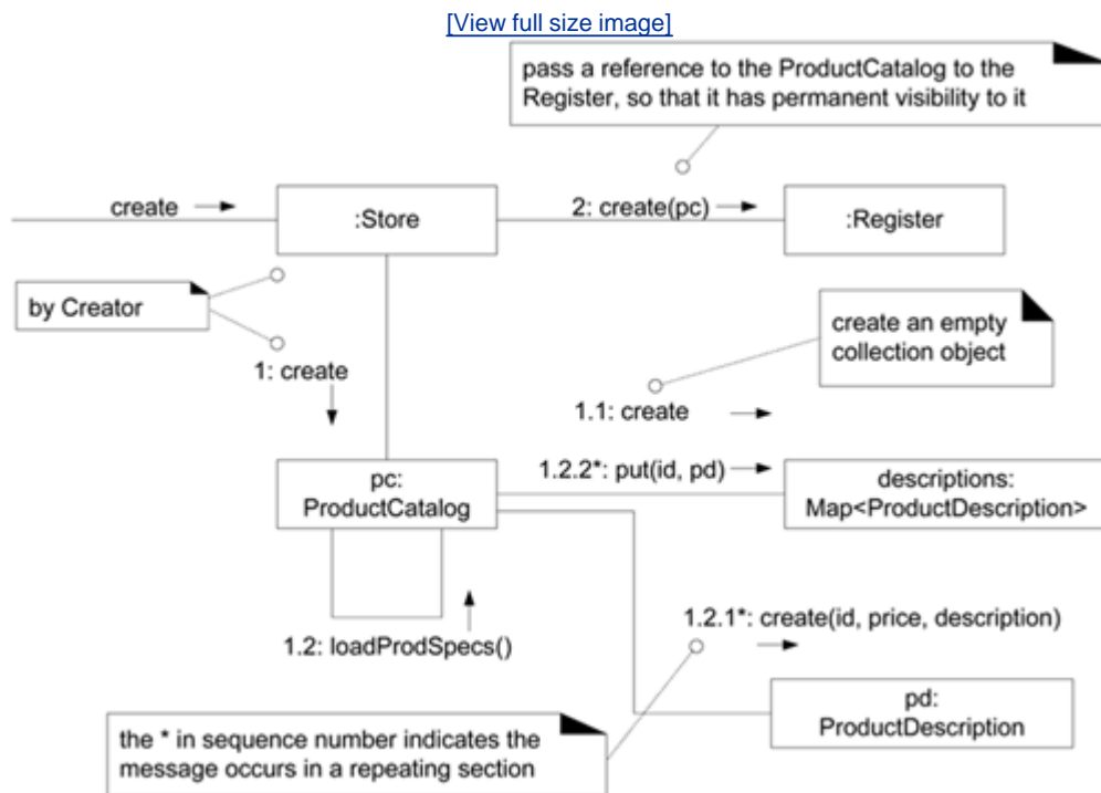
Figure 18.20. Creation of the initial domain object and subsequent objects.
