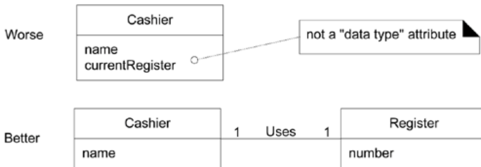
Figure 9.22. Relate with associations, not attributes.
