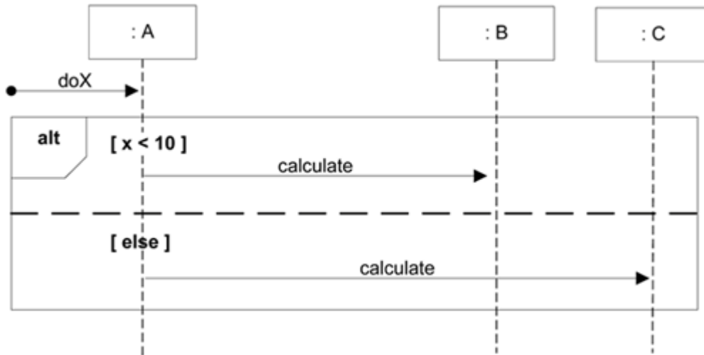
Figure 15.15. Mutually exclusive conditional messages.
