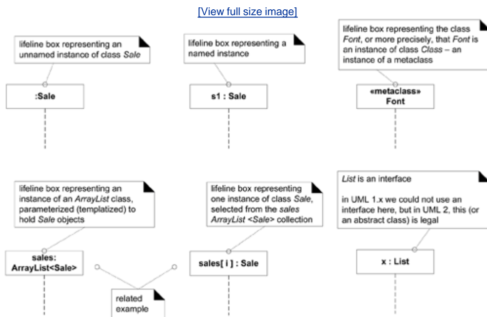
Figure 15.5. Lifeline boxes to show participants in interactions.
