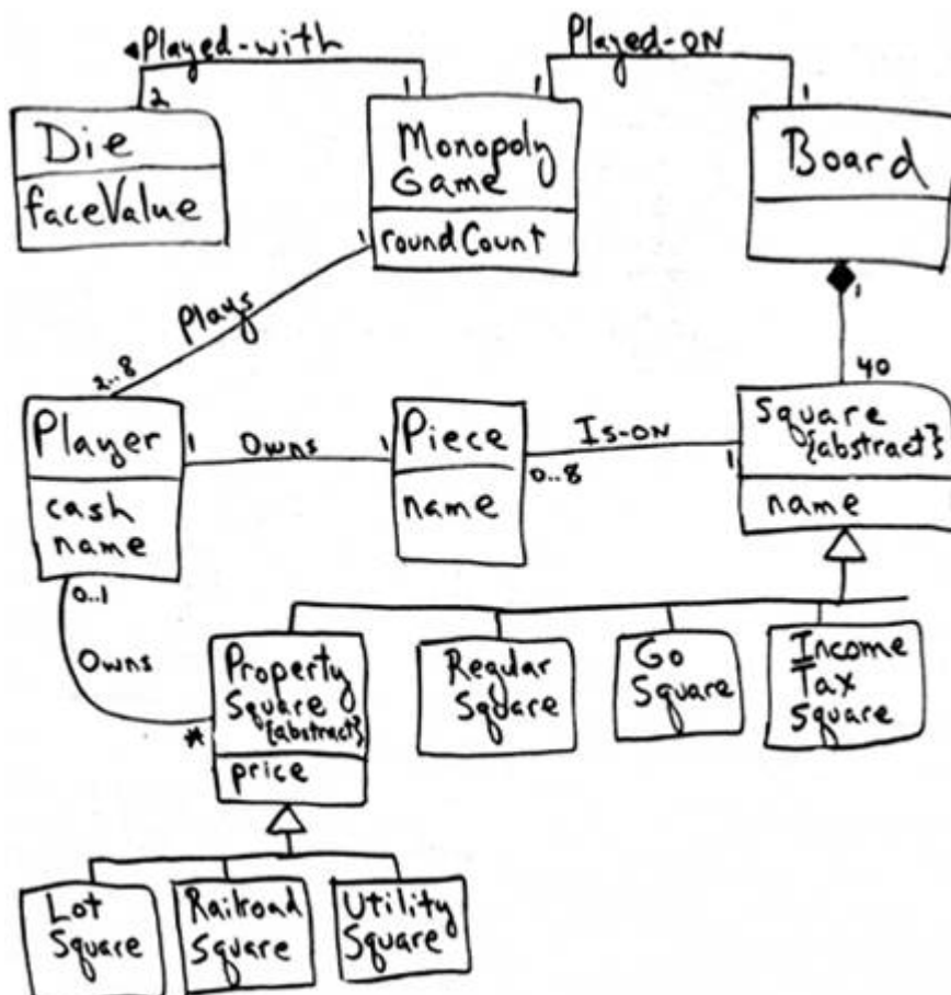
Figure 32.35. Iteration-3 Monopoly domain model.
