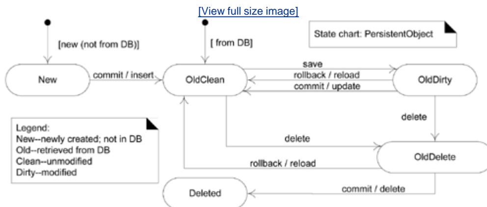
Figure 38.12. Statechart for PersistentObject.
