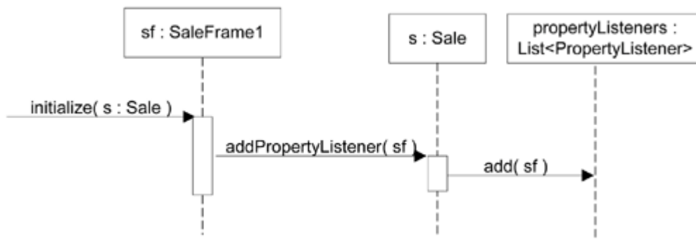
Figure 26.23. The observer SaleFrame1 subscribes to the publisher Sale .
