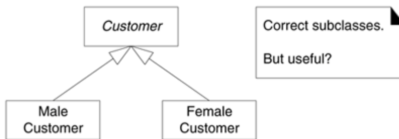
Figure 32.6. Legal conceptual class partition, but is it useful in our domain?
