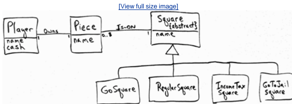
Figure 23.2. Monopoly domain model changes for iteration-2.
