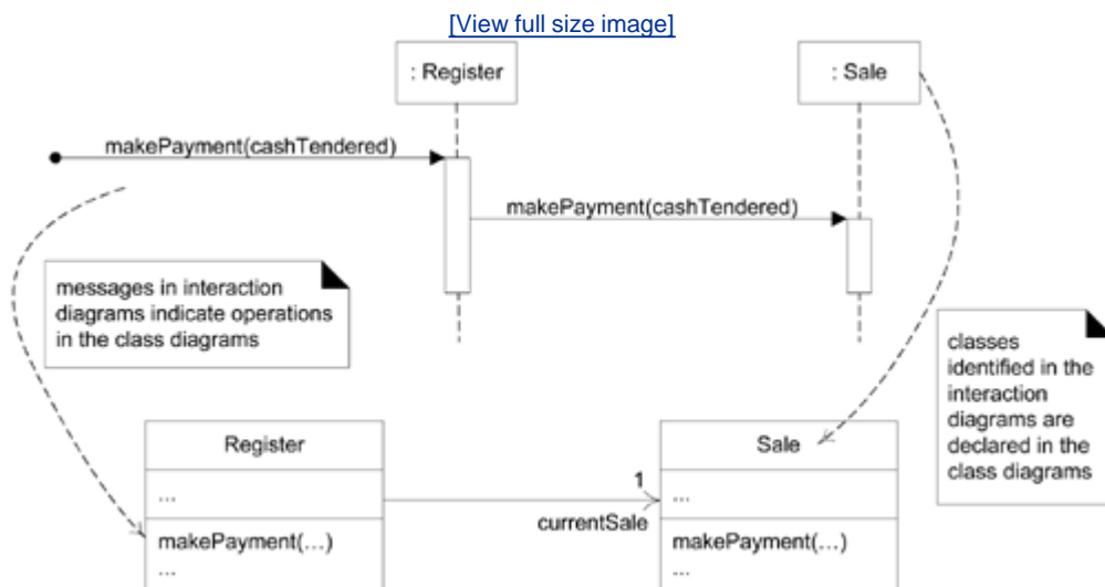
Figure 16.21. The influence of interaction diagrams on class diagrams.
