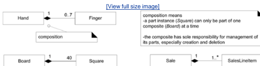
Figure 16.13. Composition in the UML.
