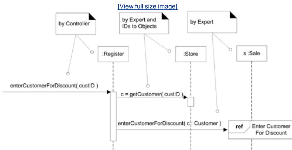
Figure 26.18. Creating the pricing strategy for a customer discount, part 1 .
