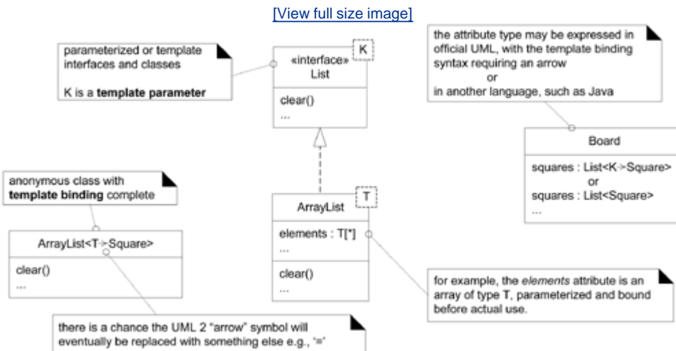
Figure 16.18. Templates in the UML.
