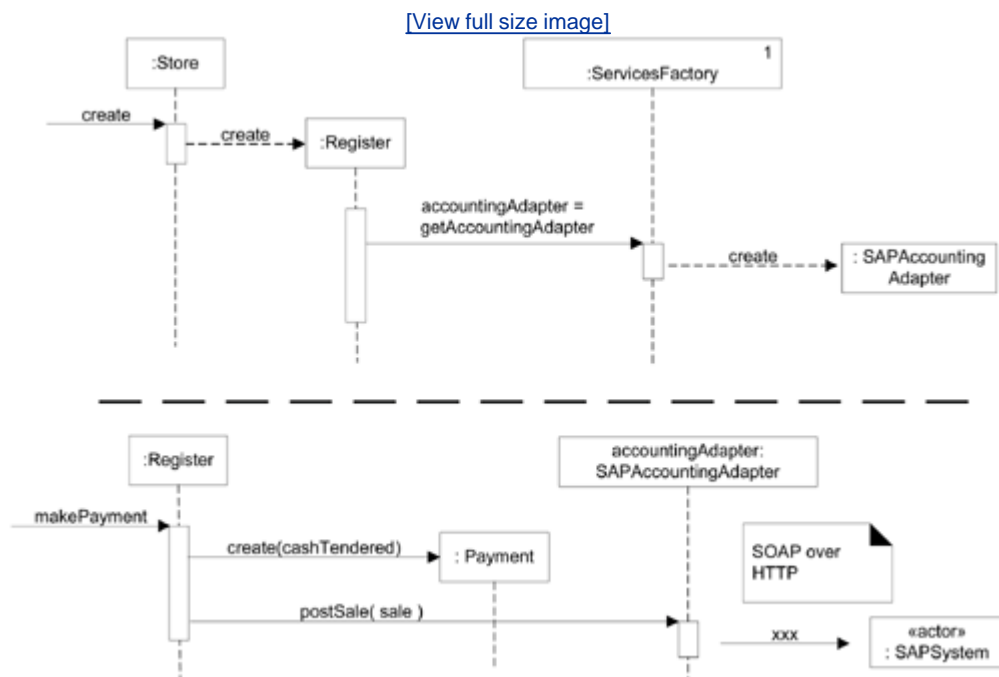
Figure 26.8. Adapter, Factory, and Singleton patterns applied to the design.
