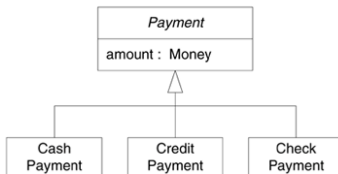
Figure 32.3. Payment class hierarchy.
