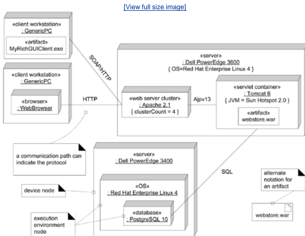
Figure 37.1. A deployment diagram.
