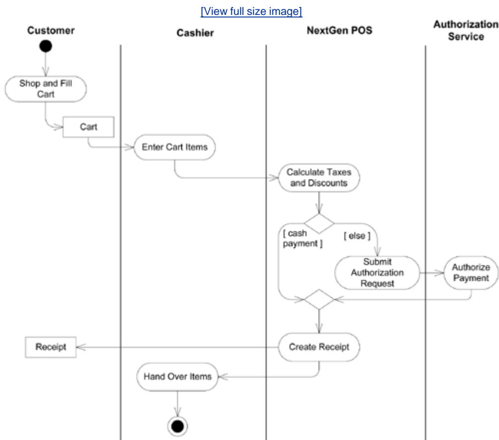
Figure 28.7. Modeling the Process Sale use case with an activity diagram.
