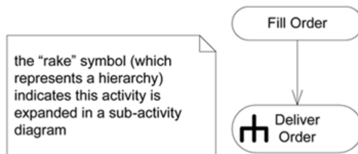
Figure 28.4. An activity will be expanded in another diagram.
