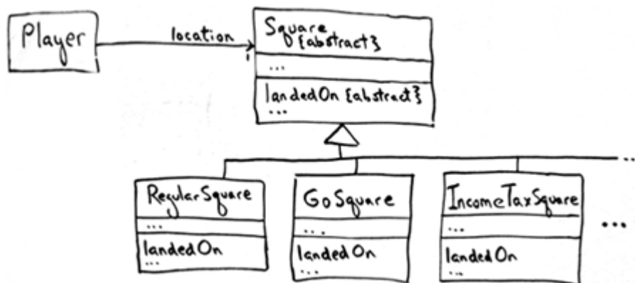
Figure 35.23. DCD for the polymorphic landedOn design strategy.
