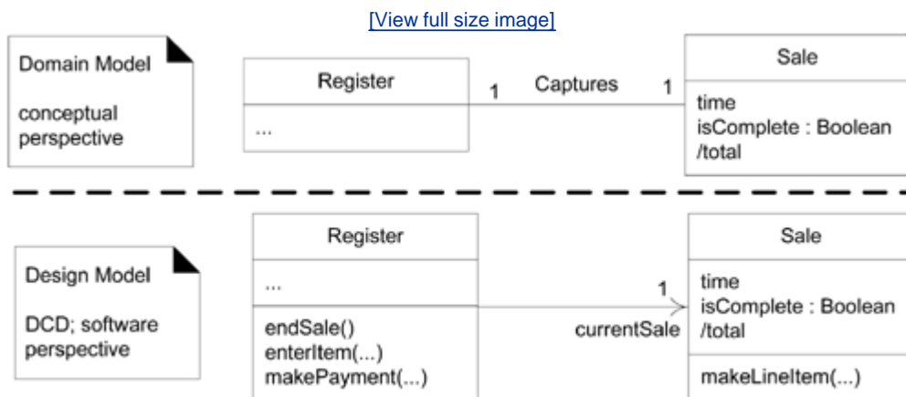
Figure 16.2. UML class diagrams in two perspectives.
