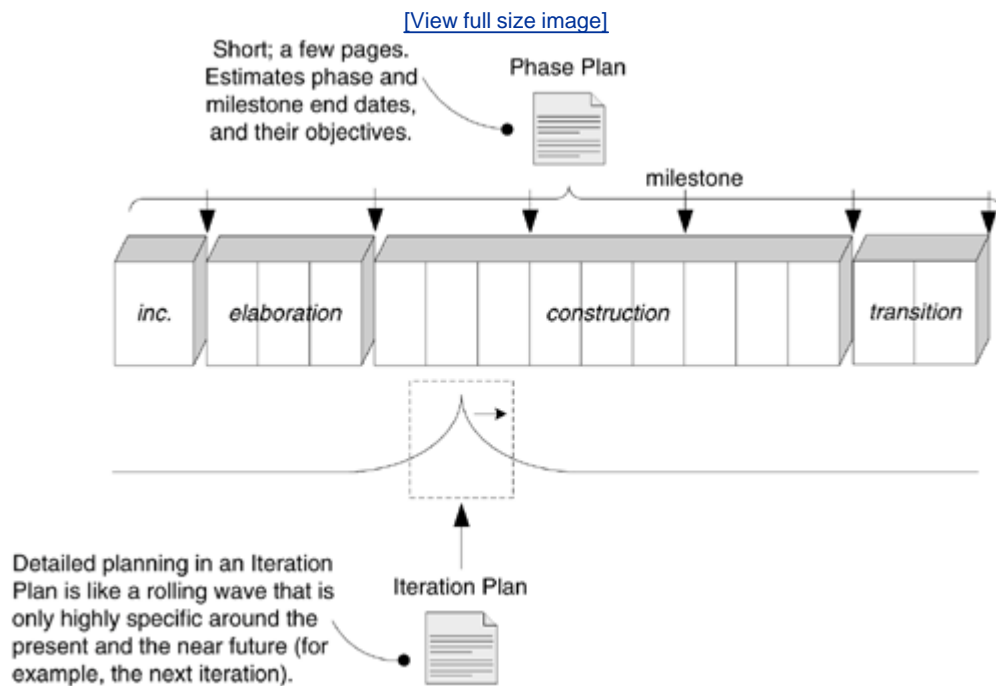
Figure 40.2. Phase and Iteration Plans.
