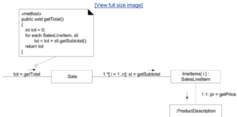
Figure 18.11. Showing a method in a note symbol.
