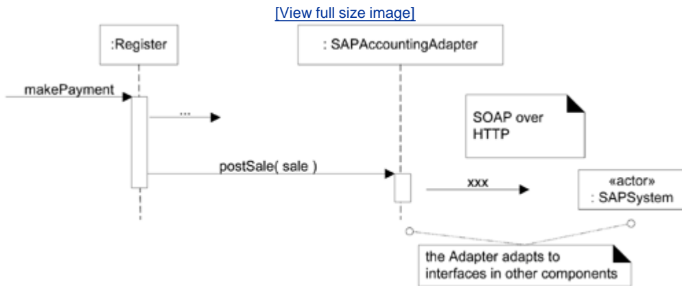
Figure 26.2. Using an Adapter.
