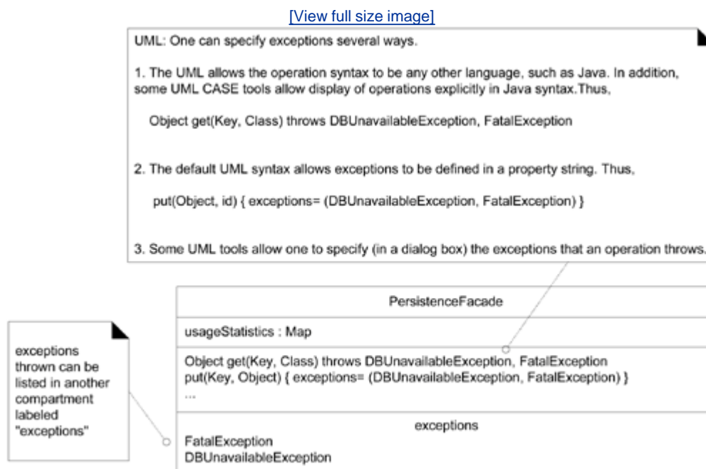
Figure 35.9. Exceptions caught and thrown by a class.
