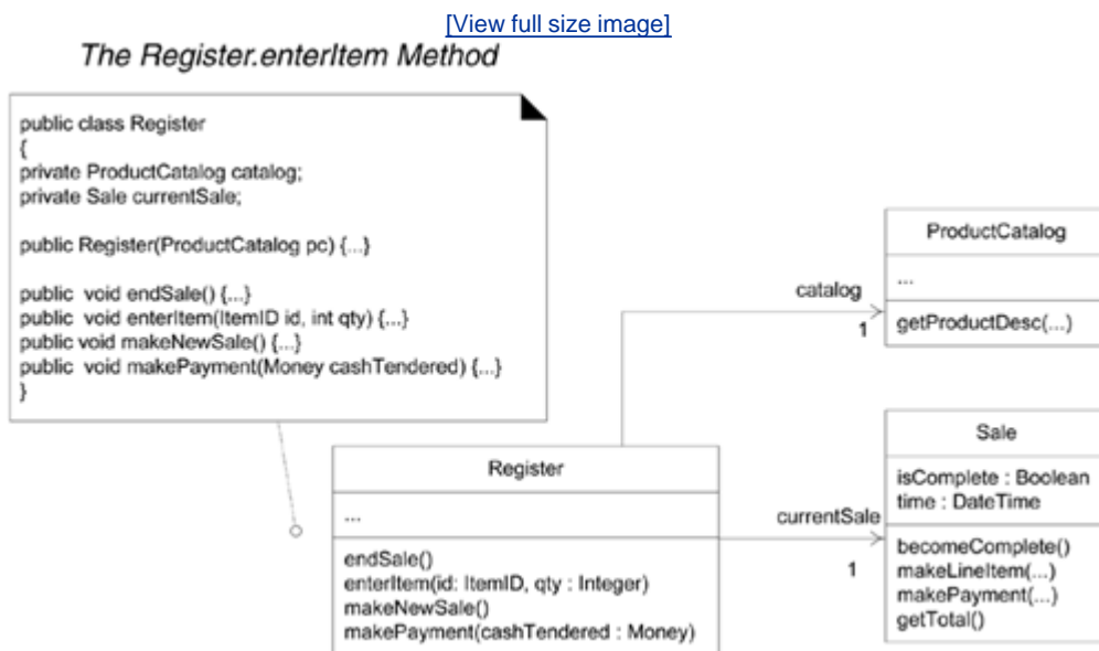
Figure 20.3. The Register class.
