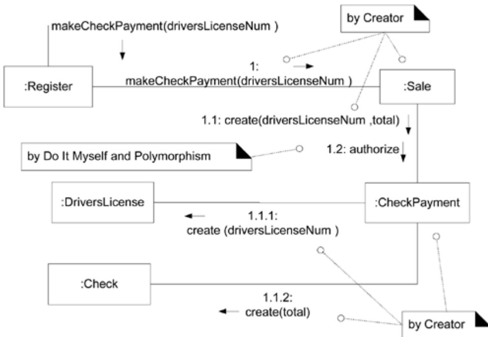
Figure 35.19. Creating a CheckPayment.
