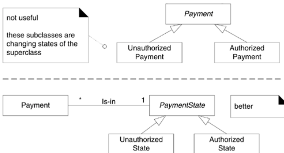
Figure 32.13. Modeling changing states.
