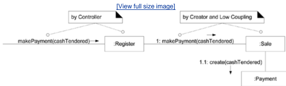
Figure 18.13. Register.makePayment interaction diagram.
