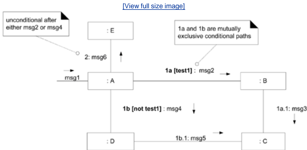
Figure 15.30. Mutually exclusive messages.
