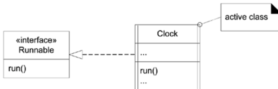
Figure 16.20. Active classes in the UML.
