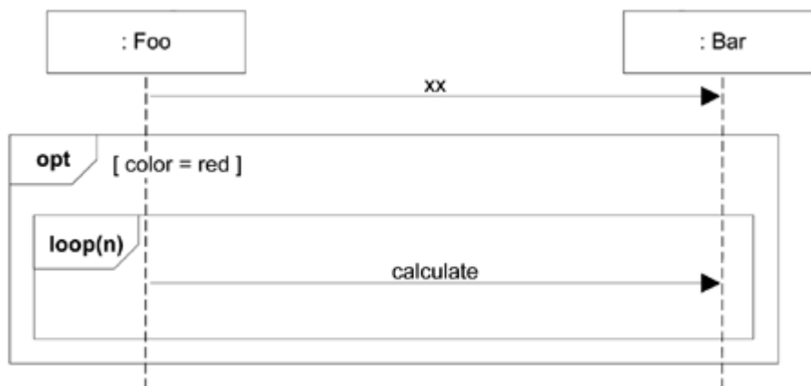
Figure 15.18. Nesting of frames.
