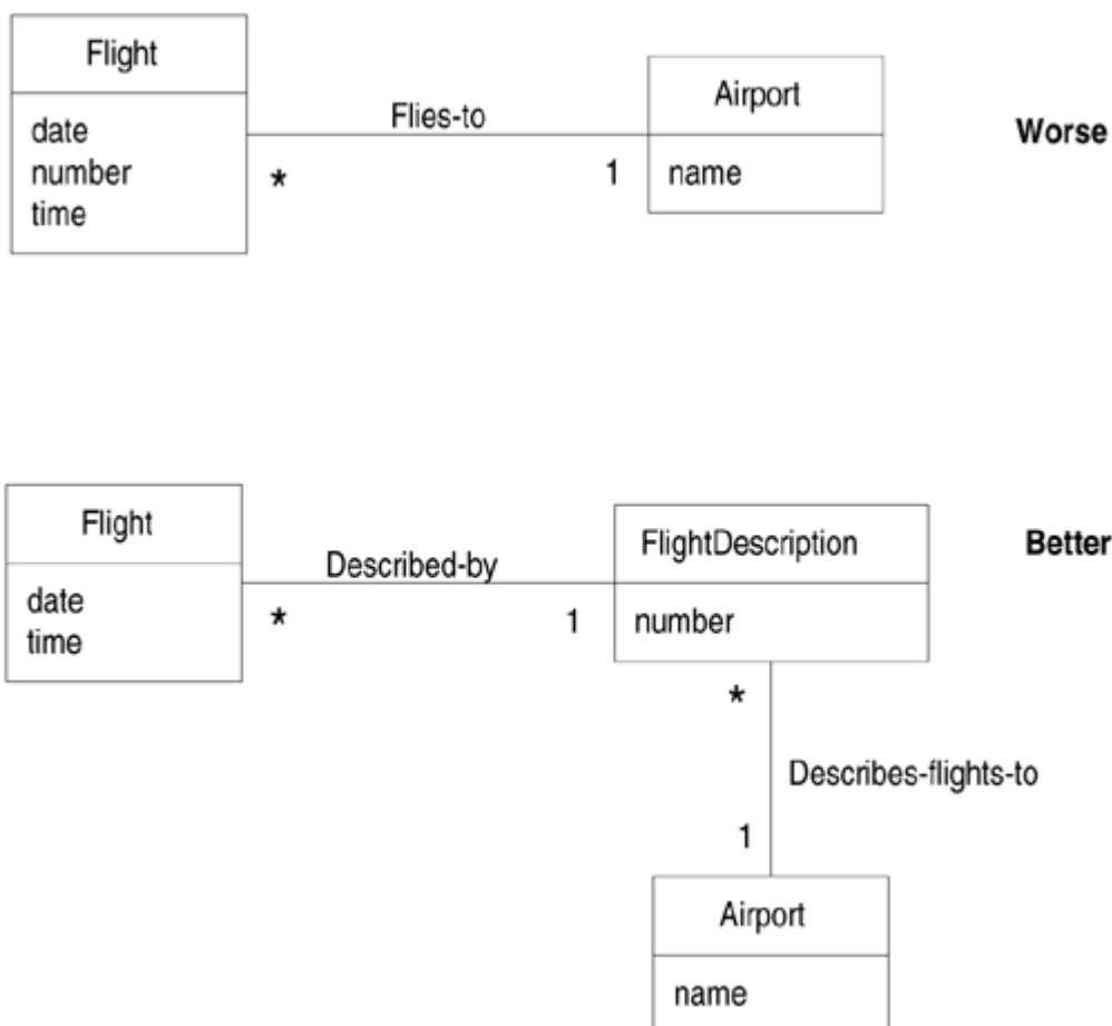
Figure 9.10. Descriptions about other things.
