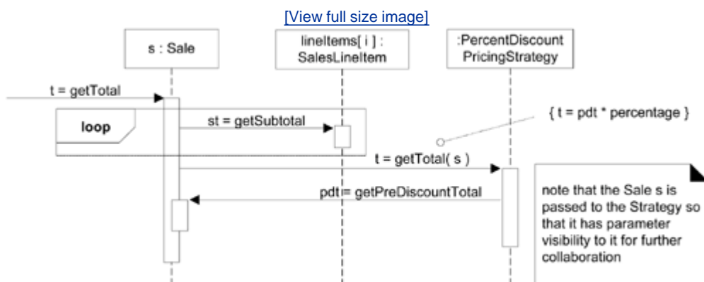
Figure 26.10. Strategy in collaboration.
