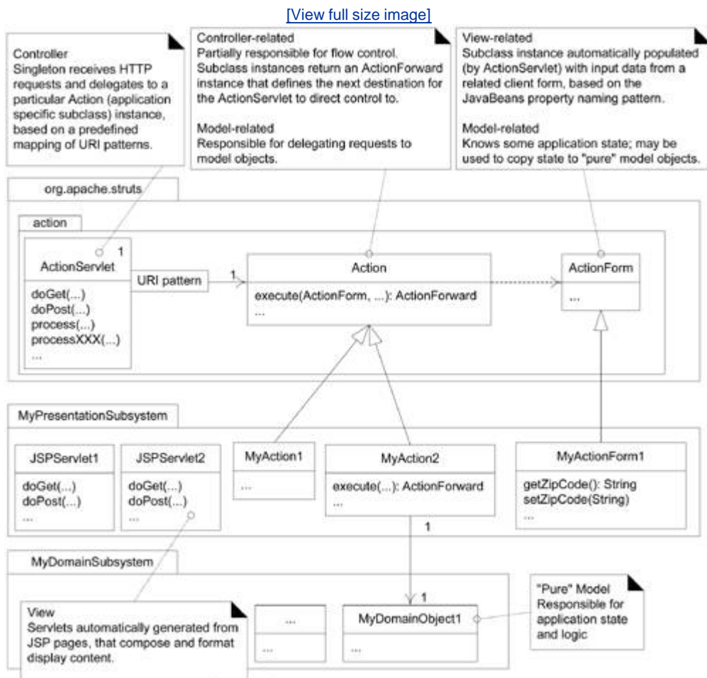
Figure 2. MVC roles in Struts.
