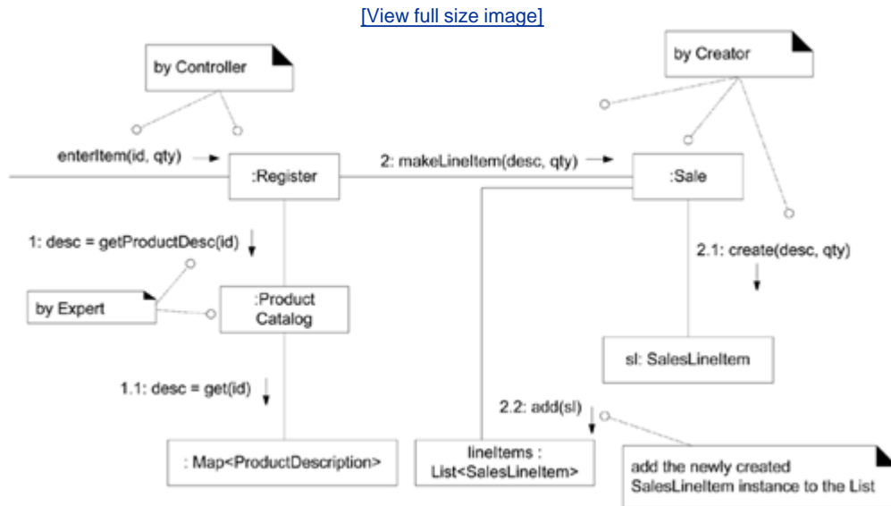
Figure 18.7. The enterItem interaction diagram. Dynamic view.
