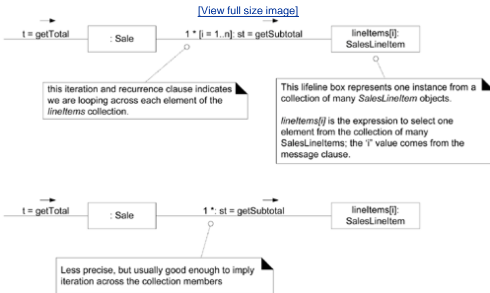
Figure 15.32. Iteration over a collection.
