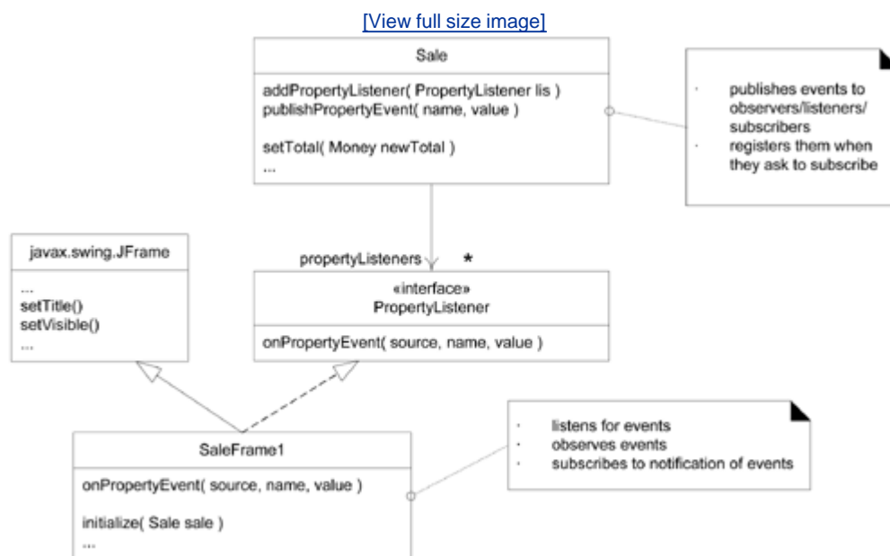
Figure 26.26. Who is the observer, listener, subscriber, and publisher?
