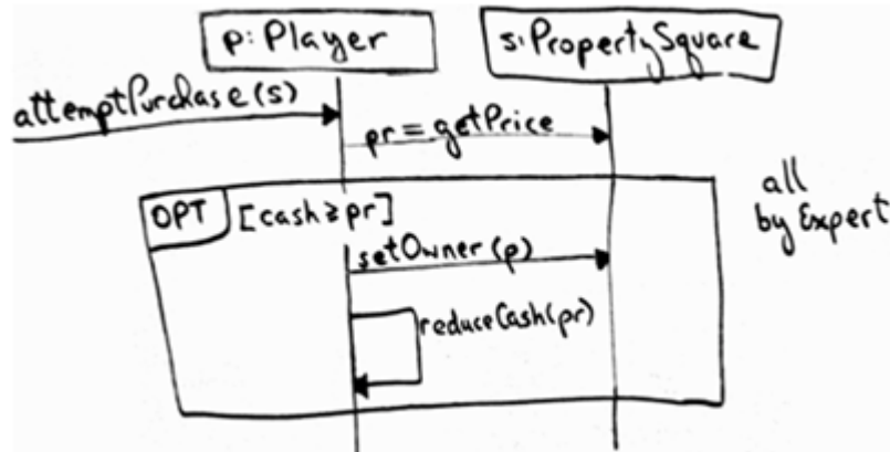
Figure 35.26. Attempting to purchase a property.
