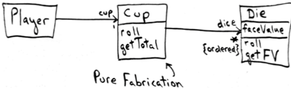
Figure 25.8. DCD for a Cup .
