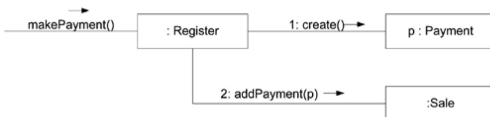
Figure 17.18. Register creates Payment.
