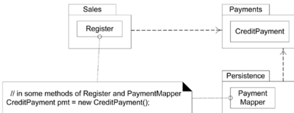
Figure 36.3. Direct coupling to concrete package due to creation.
