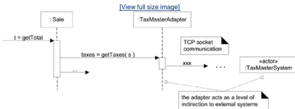
Figure 25.10. Indirection via the adapter.
