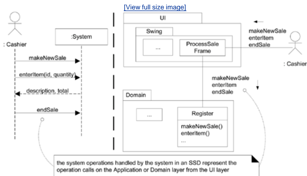
Figure 34.9. System operations in the SSDs and in terms of layers.
