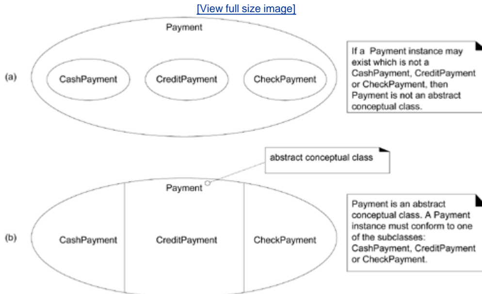
Figure 32.11. Abstract conceptual classes.
