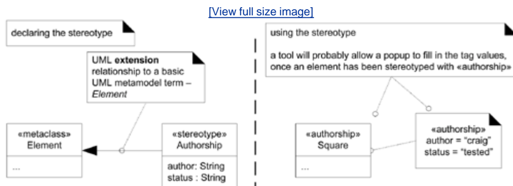
Figure 16.8. Stereotype declaration and use.
