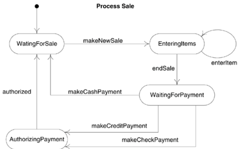
Figure 29.5. A sample state machine for legal sequence of use case operations.
