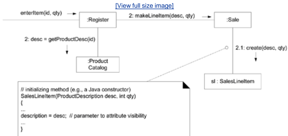
Figure 19.4. Parameter to attribute visibility.
