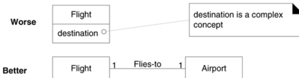
Figure 9.23. Don't show complex concepts as attributes; use associations.
