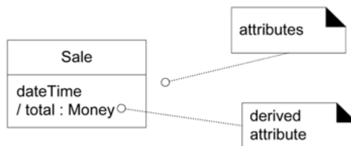
Figure 9.19. Class and attributes.
