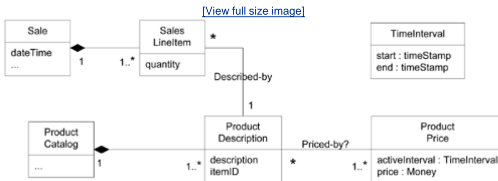
Figure 32.19. Product Prices and time intervals.
