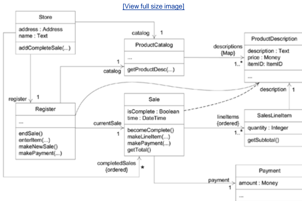
Figure 18.17. A more complete DCD reflecting most design decisions.
