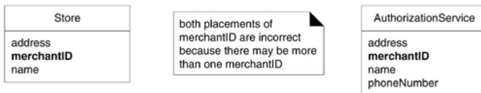
Figure 32.14. Inappropriate use of an attribute.
