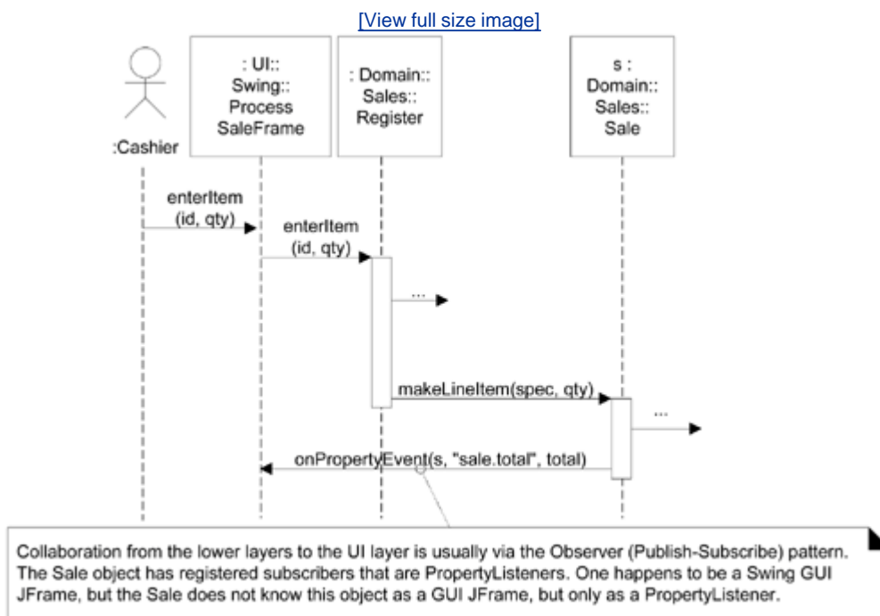
Figure 34.10. Observer for "upward" communication to the UI layer.
