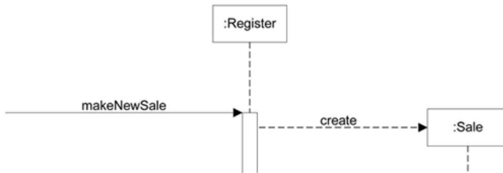
Figure 18.5. Applying the GRASP Controller pattern.
