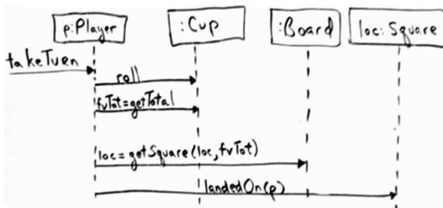
Figure 35.24. Dynamic collaborations for the landedOn design strategy.
