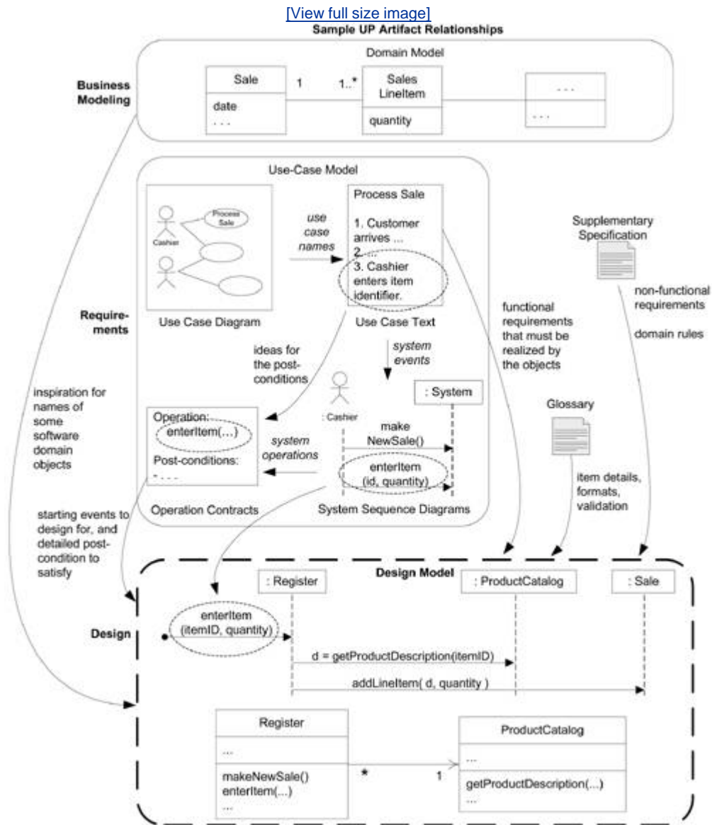
Figure 17.1. Artifact relationships emphasizing influence on OO design.
