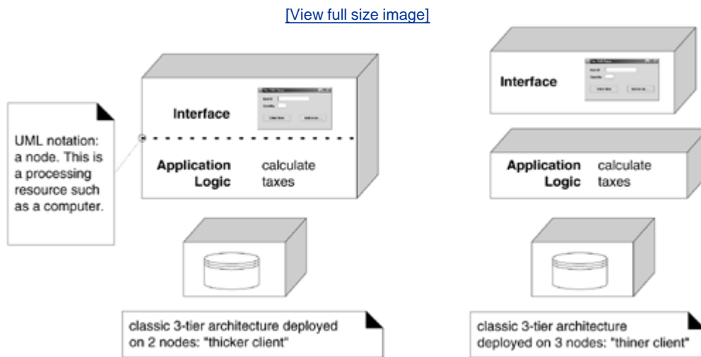
Figure 34.12. A three-tier logical division deployed in two physical architectures.
