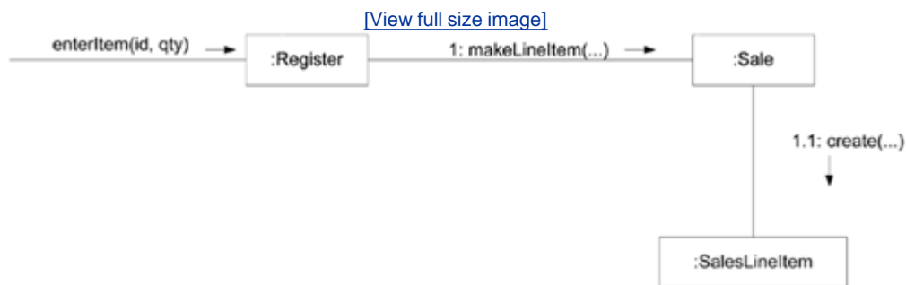
Figure 18.4. Partial interaction diagram satisfies a contract postcondition.
