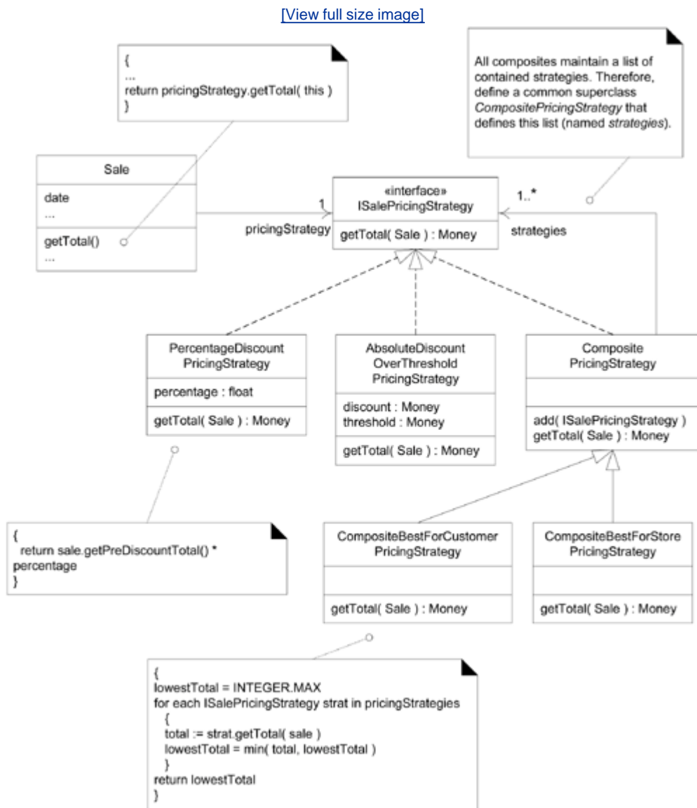
Figure 26.14. The Composite pattern.
