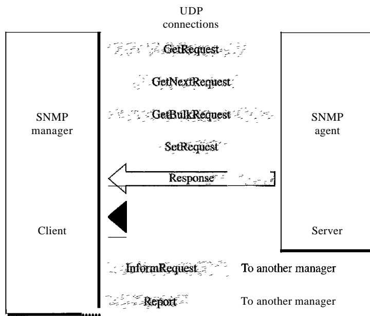
Figure 28.20 SNMP PDUs
