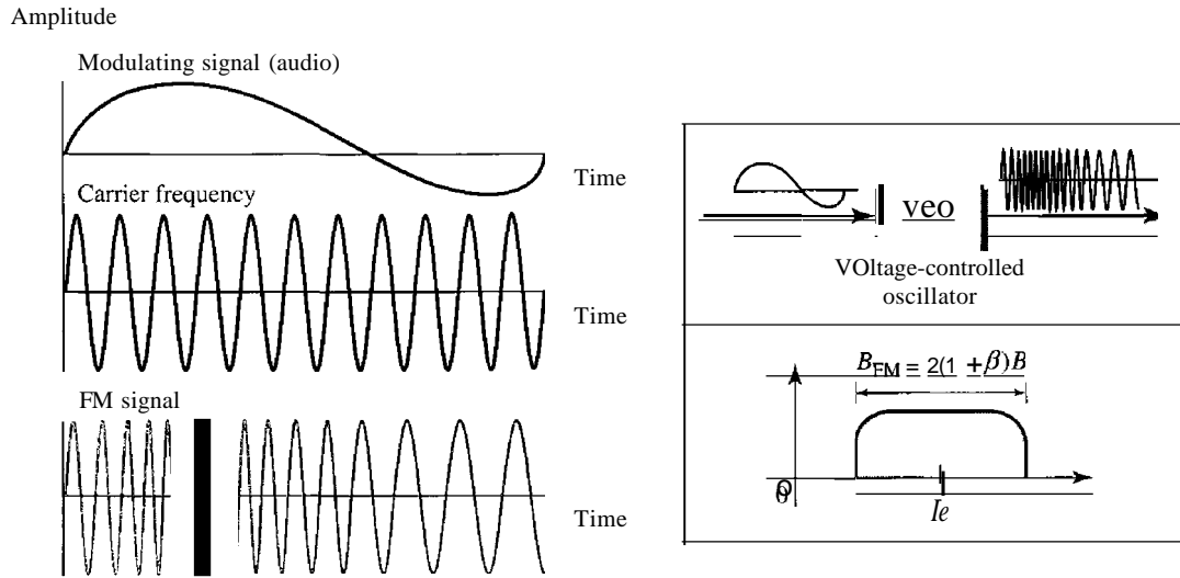
Figure 5.18 Frequency modulation
