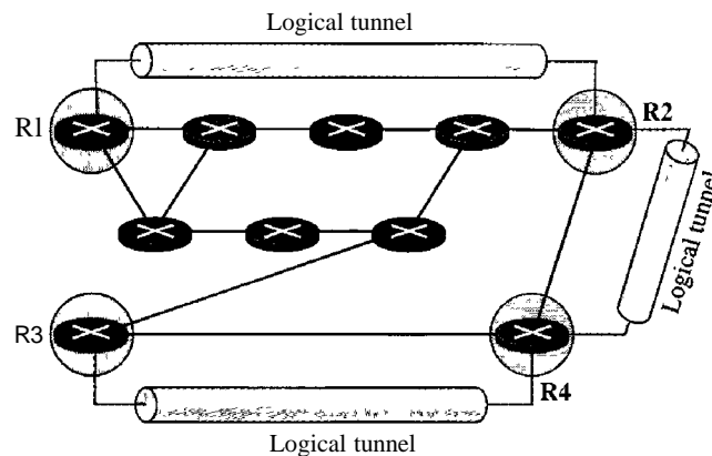
Figure 22.46 Logical tunneling
