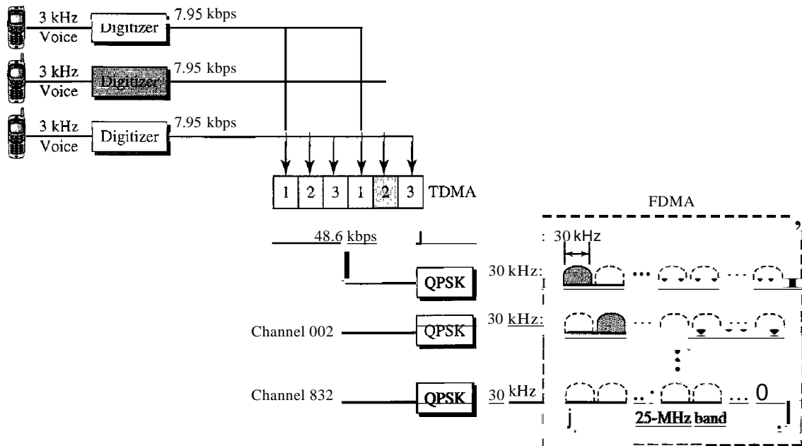
Figure 16.6 D-AMPS
