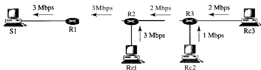
Figure 24.24 Reservation merging
