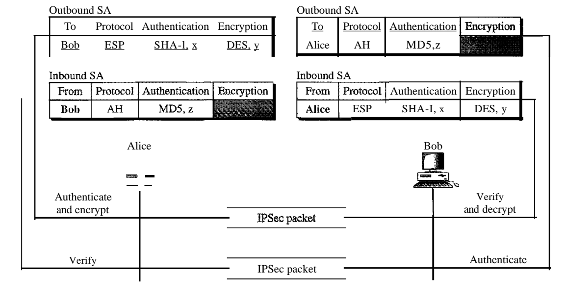
Figure 32.8 Simple inbound and outbound security associations
